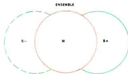
Figure 10. Typical M-S configurations rely on a cardioid microphone for the mid, and a bi-directional microphone for the side signals.
