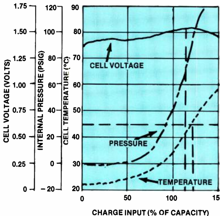
Figure 19. NiCad curves of temperature, voltage and pressure during charge.
