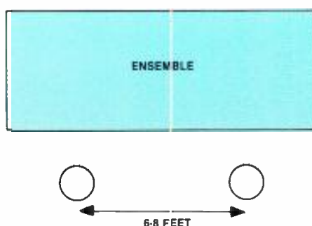
Figure 2. The spaced microphone technique is simple, but often produces comb filtering.
