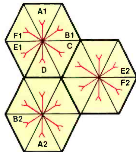
Figure 5. Sector-antenna cell splitting produces triangle-shaped cells.
