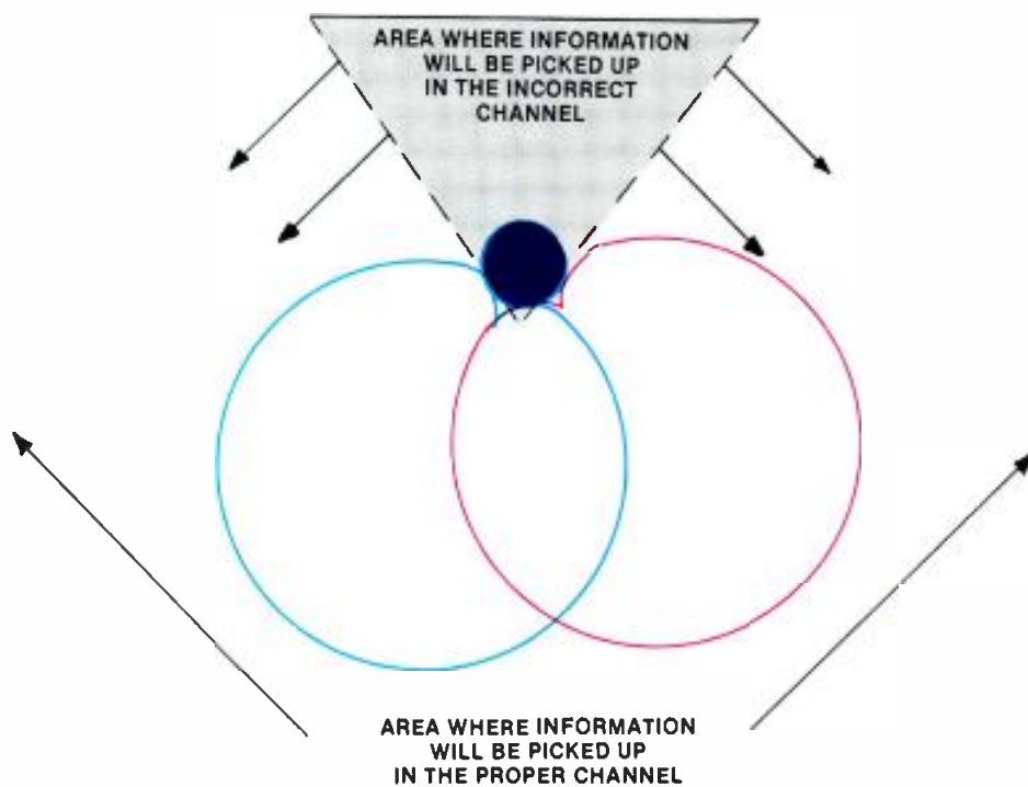
Figure 6b. A pair of crossed hypercardioid microphones provides a pickup angle of approximately 130^\circ .
