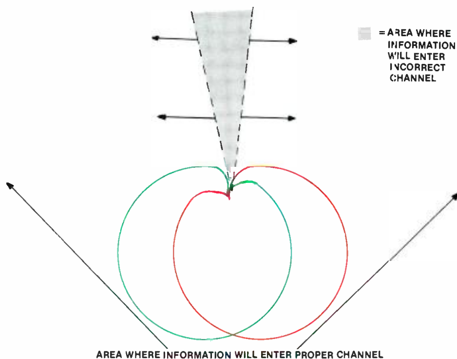
Figure 6c. Crossed cardioid microphones further increase the frontal lobe to almost 180^\circ .
