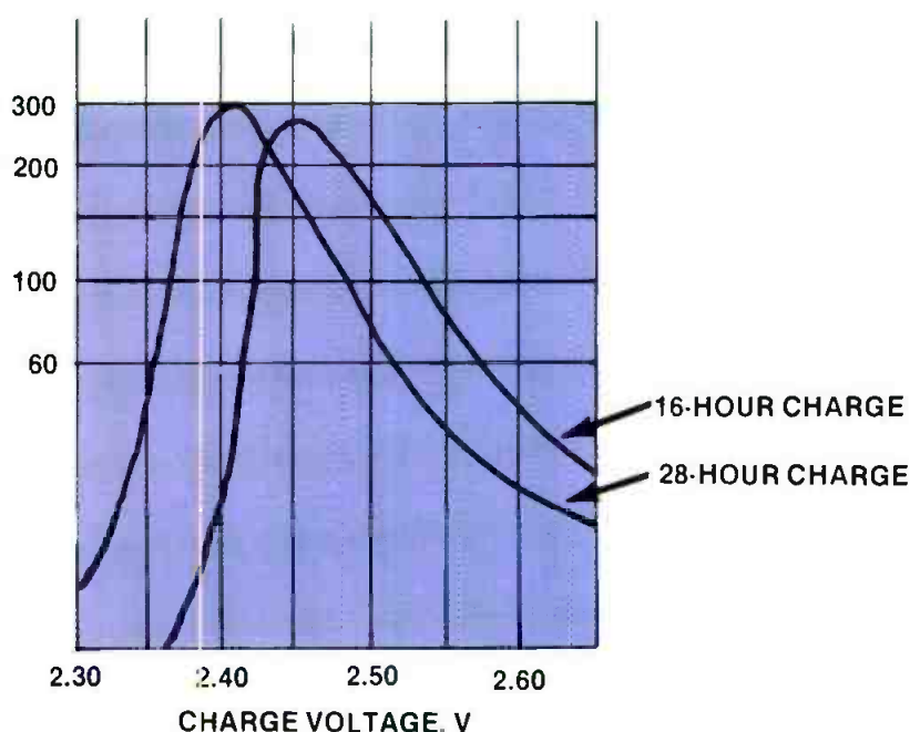
Figure 16. Lead-acid cycle life vs. charge volts.
